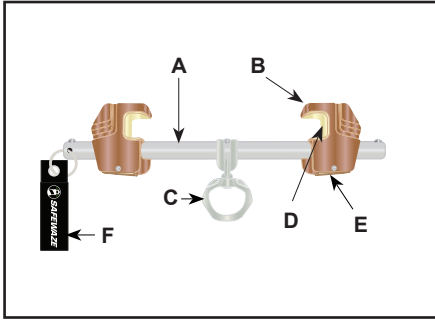
FIGURE 5 - ANCHOR COMPONENTS
