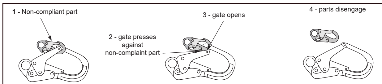
FIGURE 3 - UNINTENTIONAL DISENGAGEMENT
